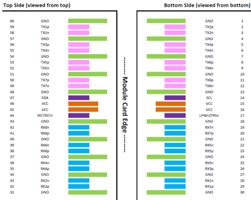
Figure 1 OSFP/OSFP-RHS Module Contact Assignment
