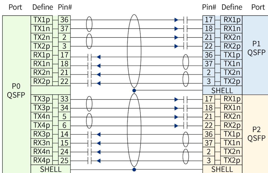
Figure 2 QSFP112 to 2*QSFP112 Direct Attached Cable assembly Wiring
