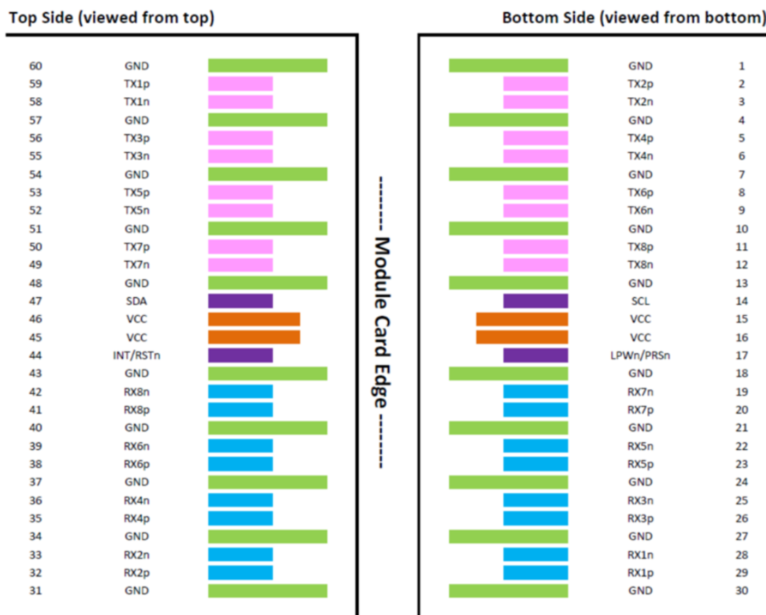
Figure 1 OSFP/OSFP RHS Type Module Contact Assignment
