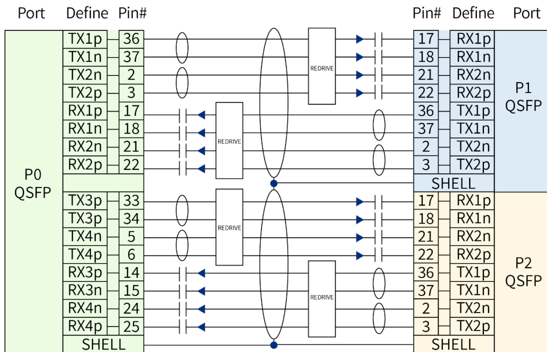
Figure 2 QSFP112 to 2*QSFP112 Active Cable assembly Wiring
