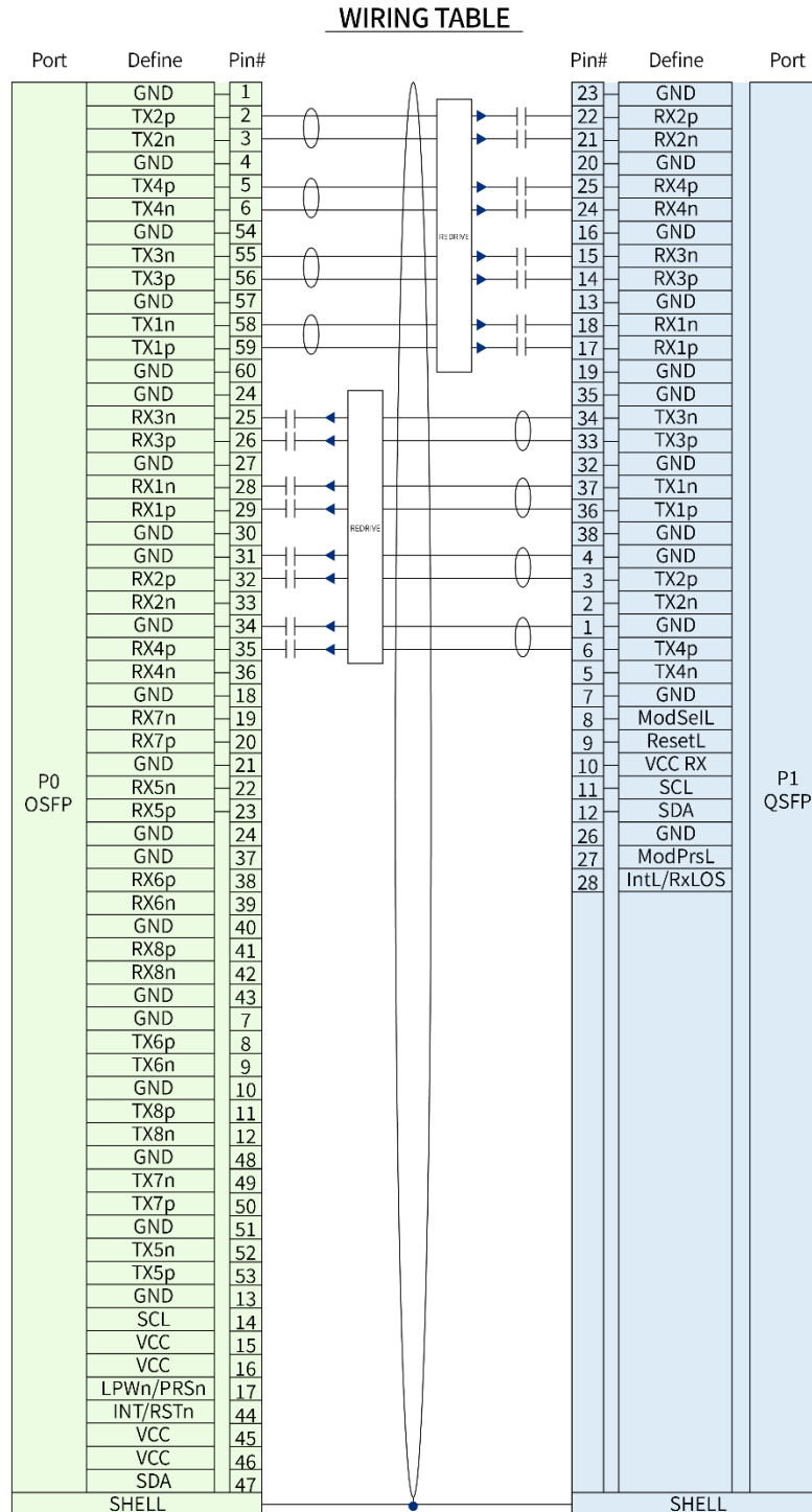
Figure 3 OSFP-RHS800 to 1*QSFP112 Active Redriver Cable Assembly Wiring
