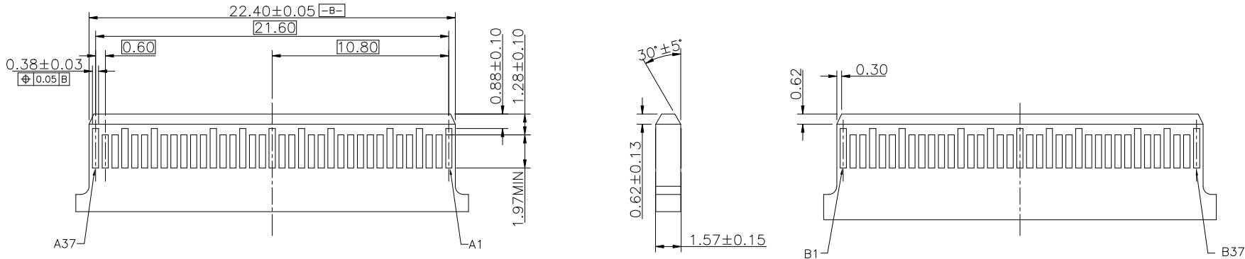
RECOMMENDED PLUG PADDLE CARD DIMENSIONS
