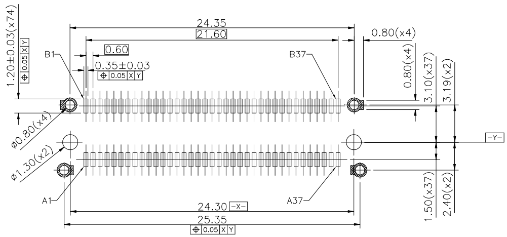
RECOMMENDED PCB LAYOUT GENERAL TOLERANCE ±0.05
