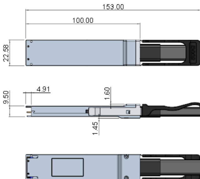
Figure 5 OSFP-RHS Type Form Factor (P1&P2 End)
